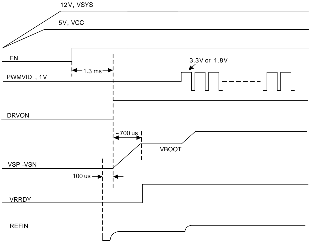
Figure 11. System Timing Diagram
