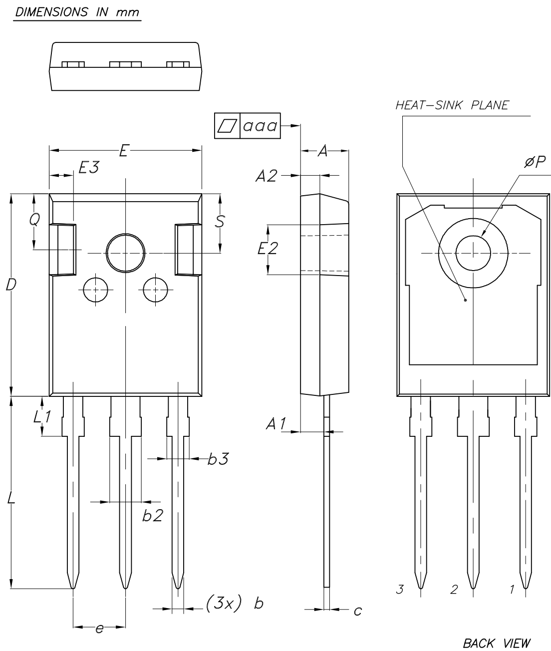
Figure 17. HiP247 long leads package outline
