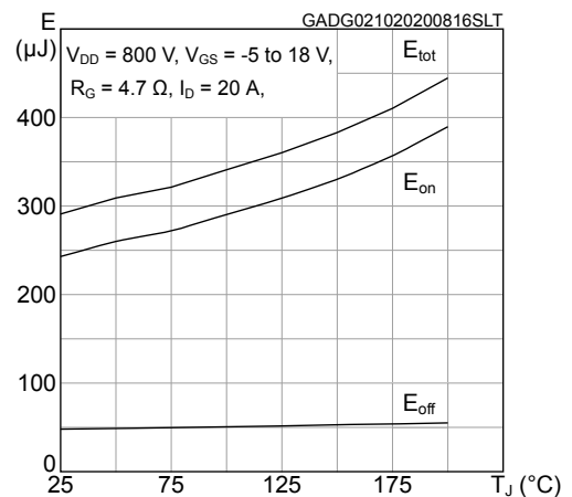
Figure 10. Typical switching energy vs junction temperature
