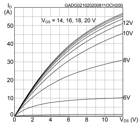
Figure 4. Typical output characteristics (T J = 200 °C)
